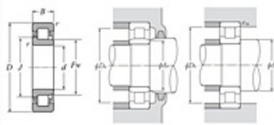
Cylindrical Roller Bearing - Separable Inner Ring w/ One Rib, Outer Ring w/ Two Ribs - NJ Type - Dimensions
