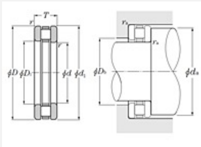
Thrust Cylindrical Roller Bearing - Type 812, 813 - Dimensions
